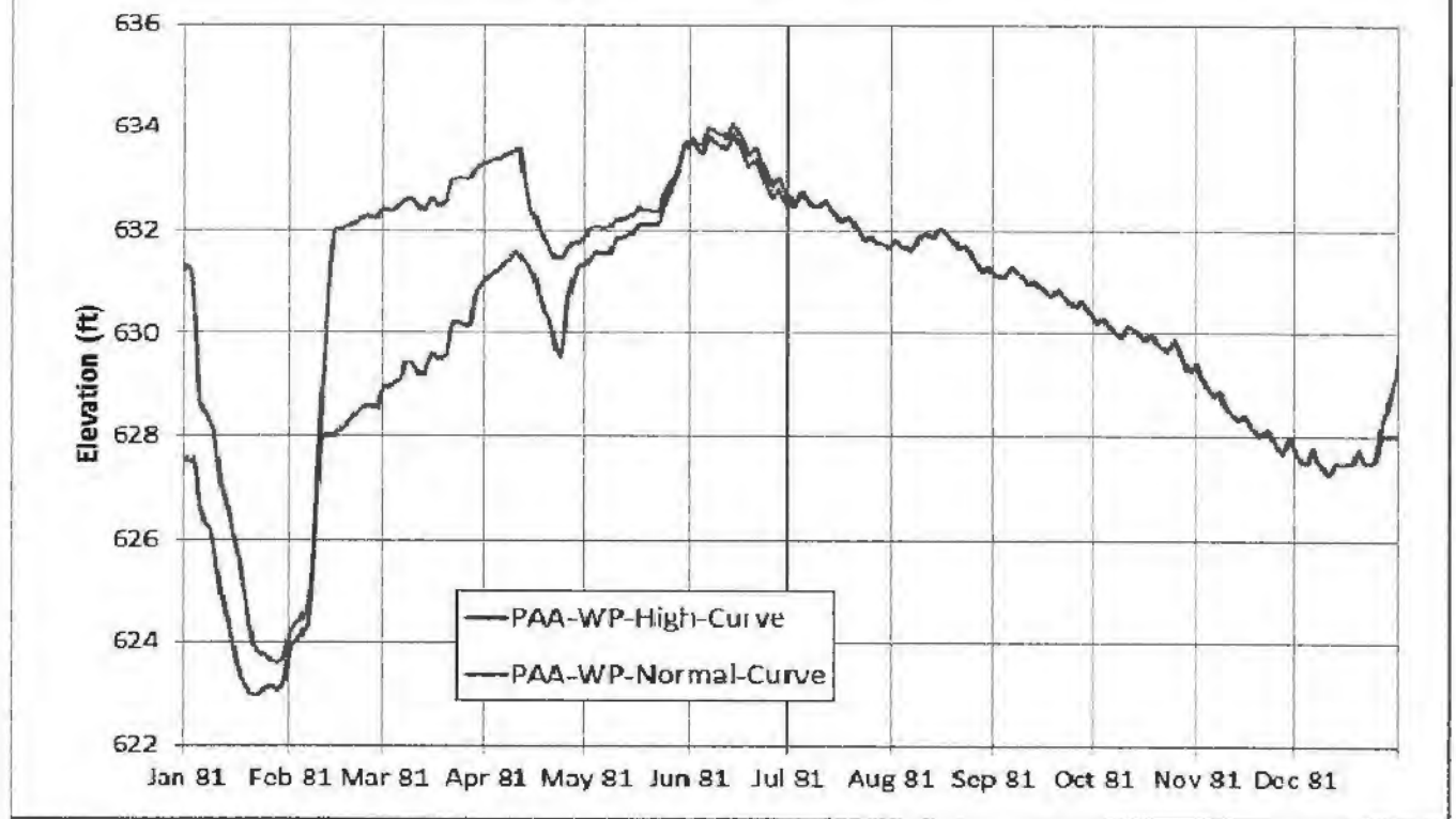
Figure 39. Simulated West Point Lake elevation in 1981.
