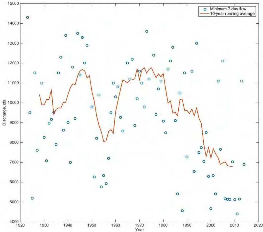
Figure 5 Minimum 7-day Low Flows for Each Year in the Apalachicola at Chattahoochee, FL
