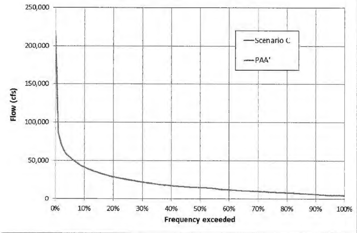
Figure 14. Duration of simulated state line flow.
