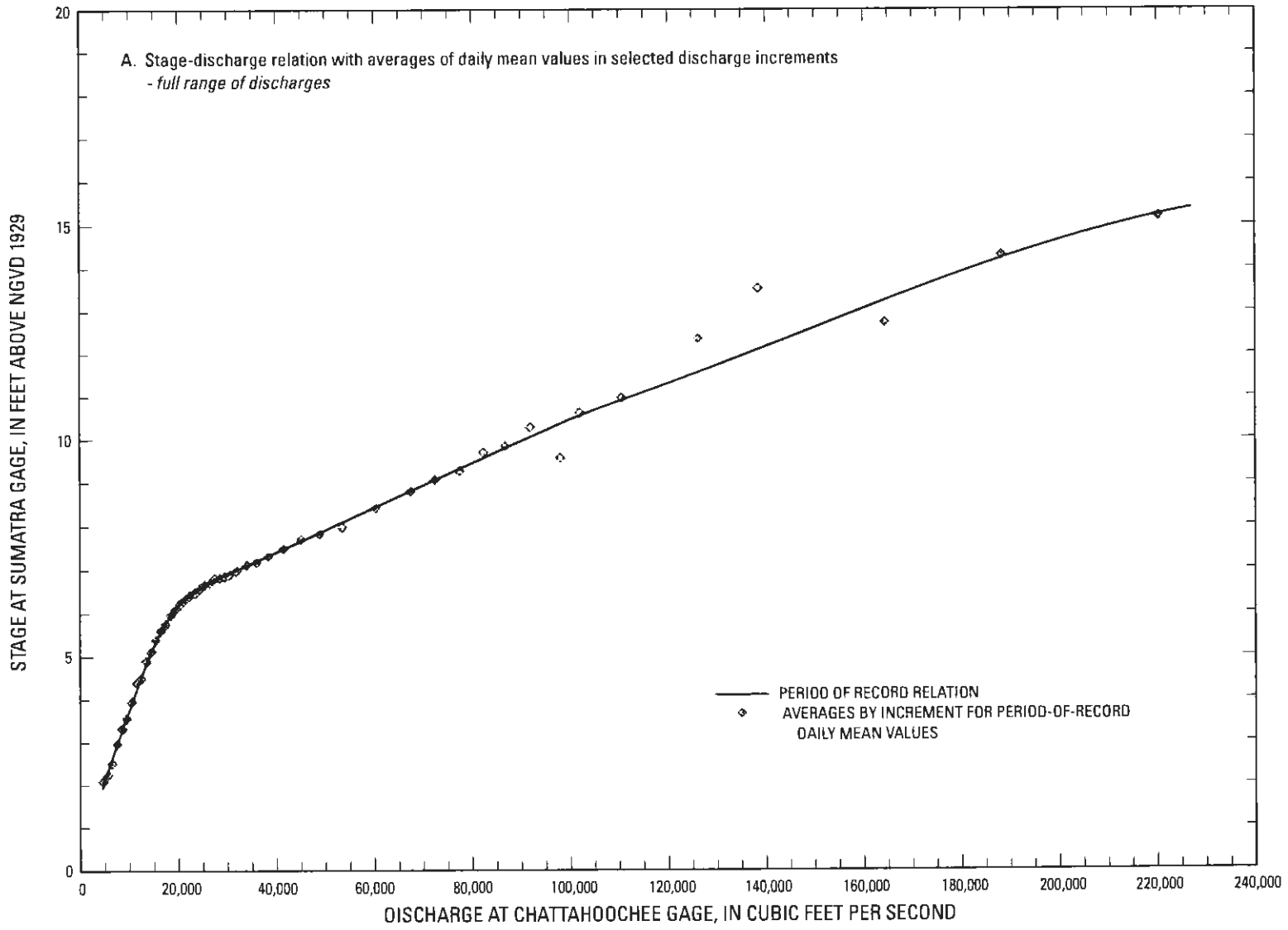
Appendix V. Stage at the Sumatra streamgage in relation to discharge at the Chattahoochee streamgage in the Apalachicola River, Florida. Relations were developed using a lag time of 3 days, as defined in glossary.
