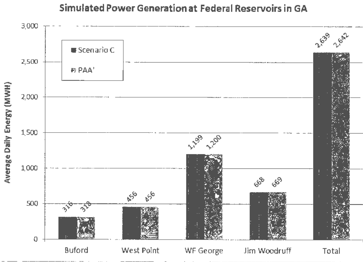
Figure 10. Simulated power generation at Federal reservoirs in Georgia.
