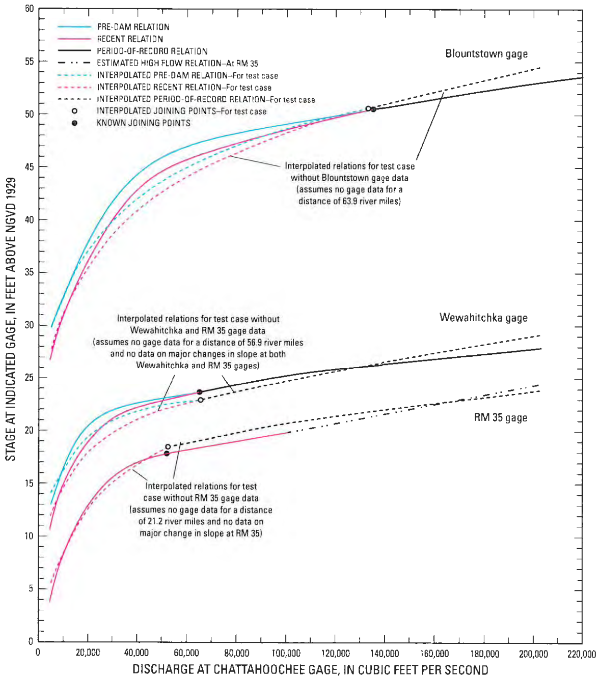
Figure 11. Stage-discharge relations based on long-term records at streamgages on the Apalachicola River, Florida, compared to hypothetical test cases in which streamgage data were ignored and relations were developed by interpolation methods used in this report. The departures shown in these hypothetical worst-case tests are greater than would be expected for the between-gage interpolated relations developed in this report (see discussion in text). Relations were developed using lag times as defined in glossary.
