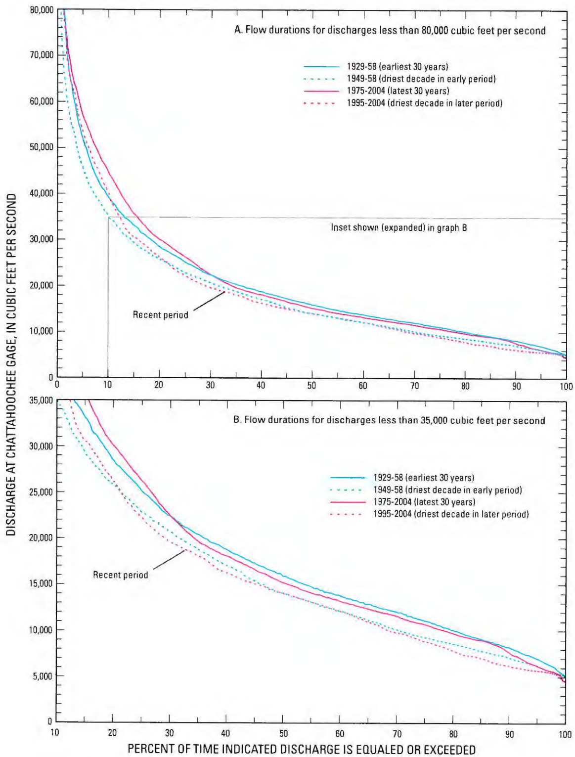
Figure 14. Flow durations for the recent period (1995–2004) compared to three other periods at the Apalachicola River at Chattahoochee, Florida, (A) for discharges less than 80,000 ft 3 /s, and (B) for discharges less than 35,000 ft 3 /s. With regard to flow durations, the recent decade including the severe drought of 1999–2002 was more similar to the decade including the severe drought of 1954–56 than it was to either of the longer 30-year periods.
