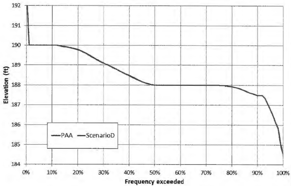
Figure 24. Duration curve of simulated W.F. George elevation
