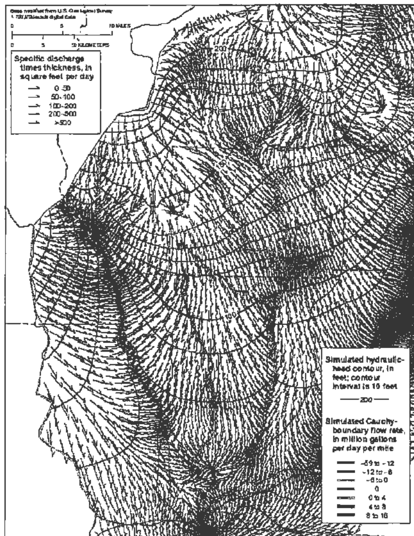
Figure 11.3: Simulated hydraulic head contours, ground-water flow direction by element, and Cauchy-boundary flow by element side in Spring Creek sub-basin for the October 1999 calibrated lower FRB model. (Jones and Torak, in review).
