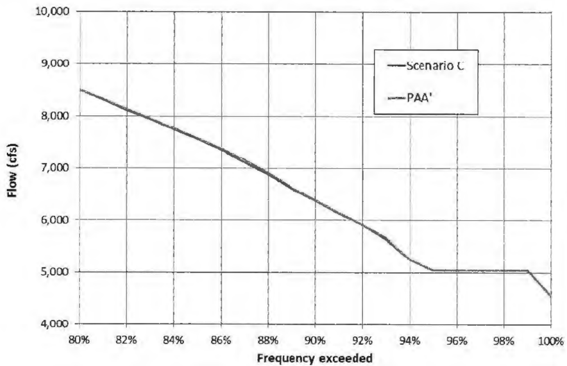
Figure 15. Duration of simulated state line flow (close-up).
