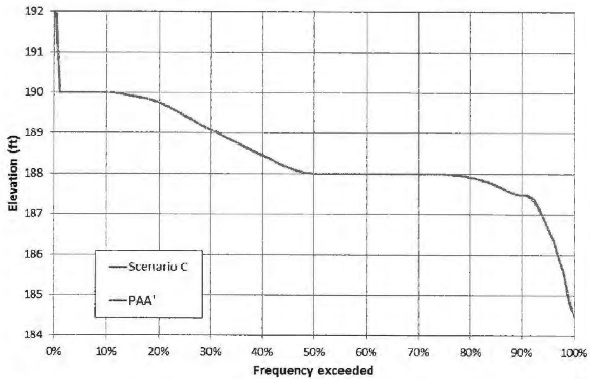
Figure 9. Duration curve of simulated W.F. George elevation.
