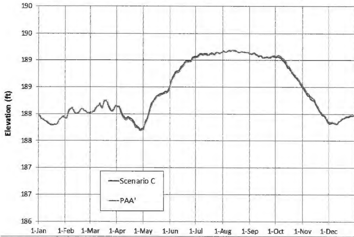
Figure 7. Simulated average daily elevation at Walter F. George Lake.
