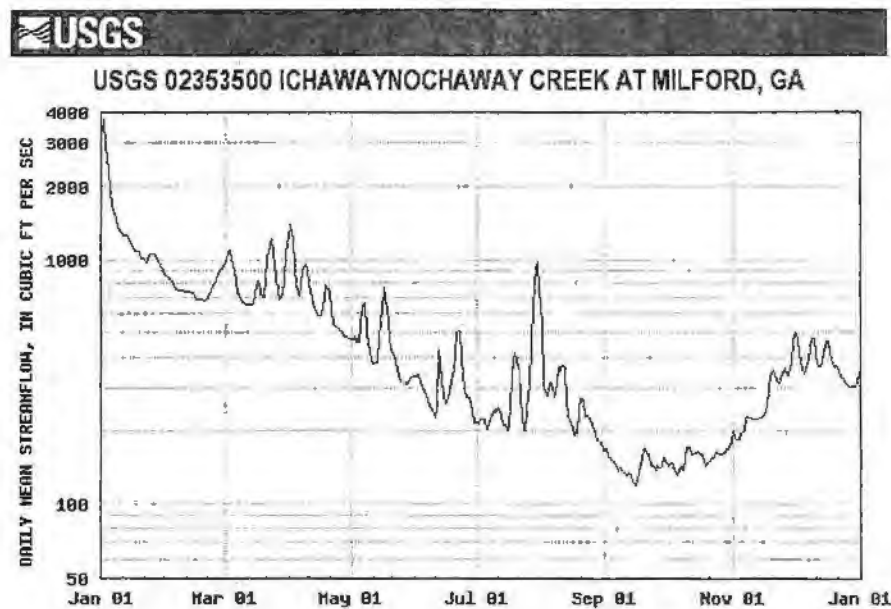
Figure 7.2. Streamflow of Ichawaynochaway Creek near Milford for 1954
