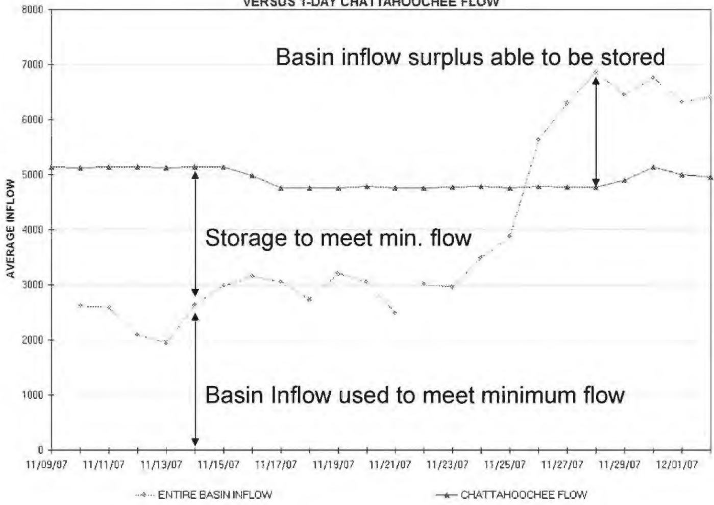
7-DAY MOVING AVERAGE INFLOW VERSUS 1-DAY CHATTAHOOCHEE FLOW
