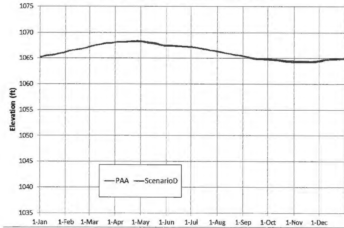
Figure 16. Simulated average daily elevation at Lanier
