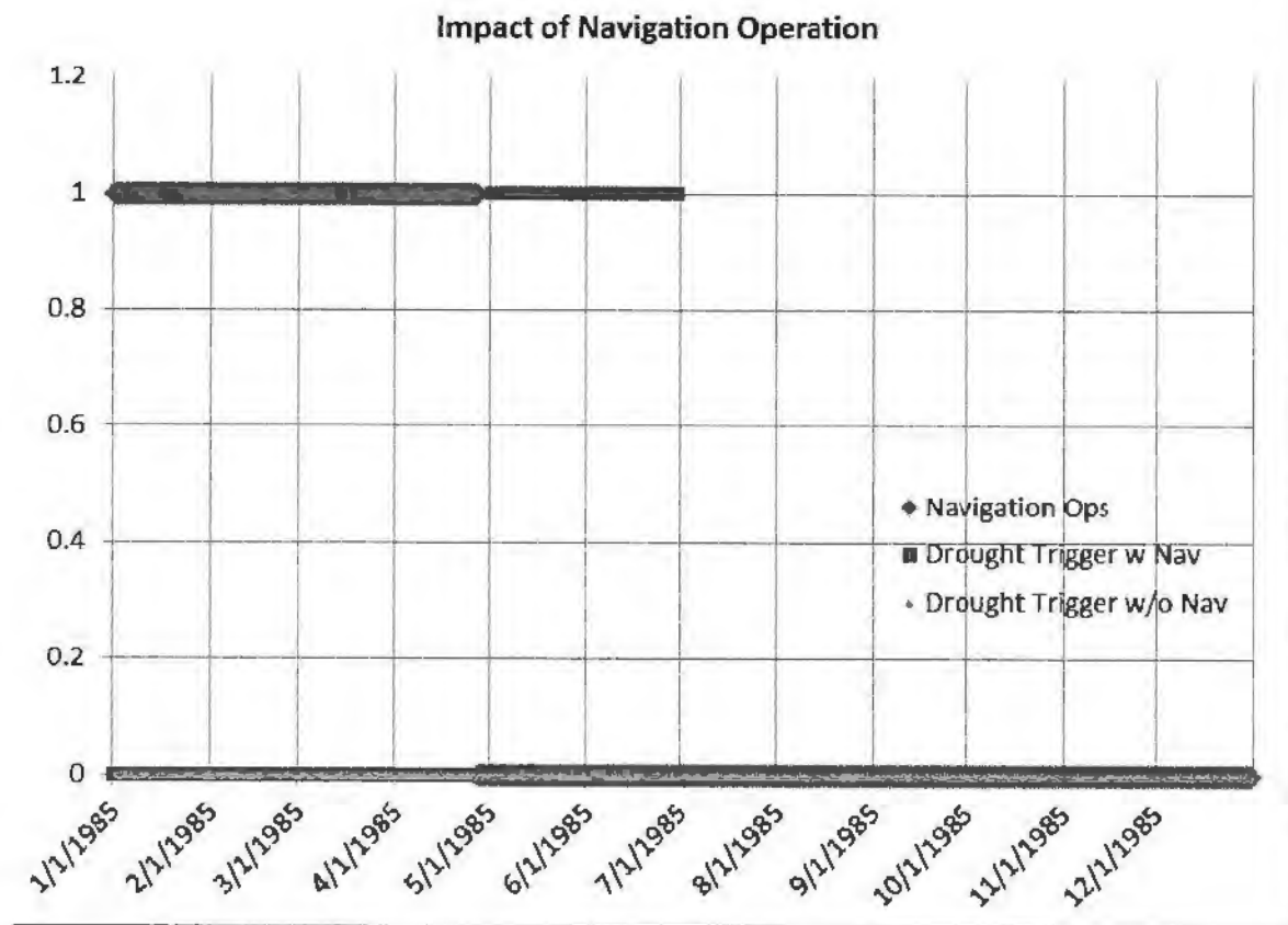
Figure 56. Additional system-wide drought operation resulting from navigation operations – 1985
