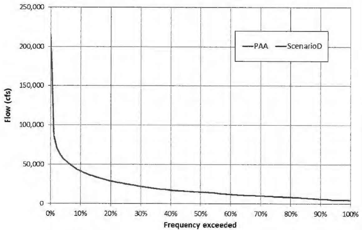
Figure 29. Duration of simulated state line flow
