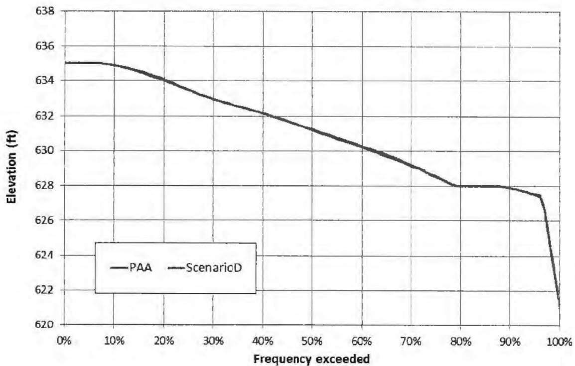
Figure 21. Duration curve of simulated West Point elevation
