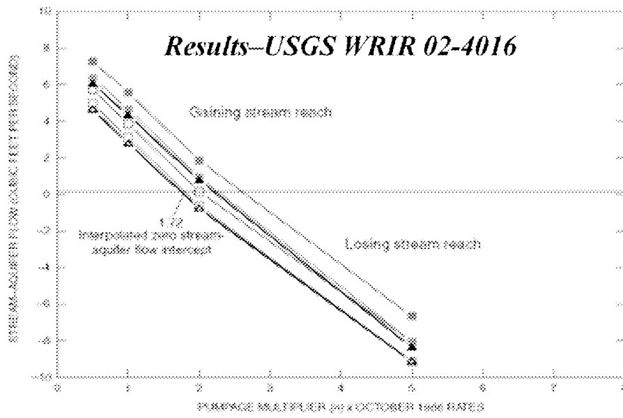
Figure B23. Stream-aquifer flow for simulated pumpage scenarios, ground-water boundary conditions, and stream stage at October 1986, Q_{50} , and Q_{10} levels for reach 23, Muskatolee Creek, Georgia (see fig. 8 for location).
