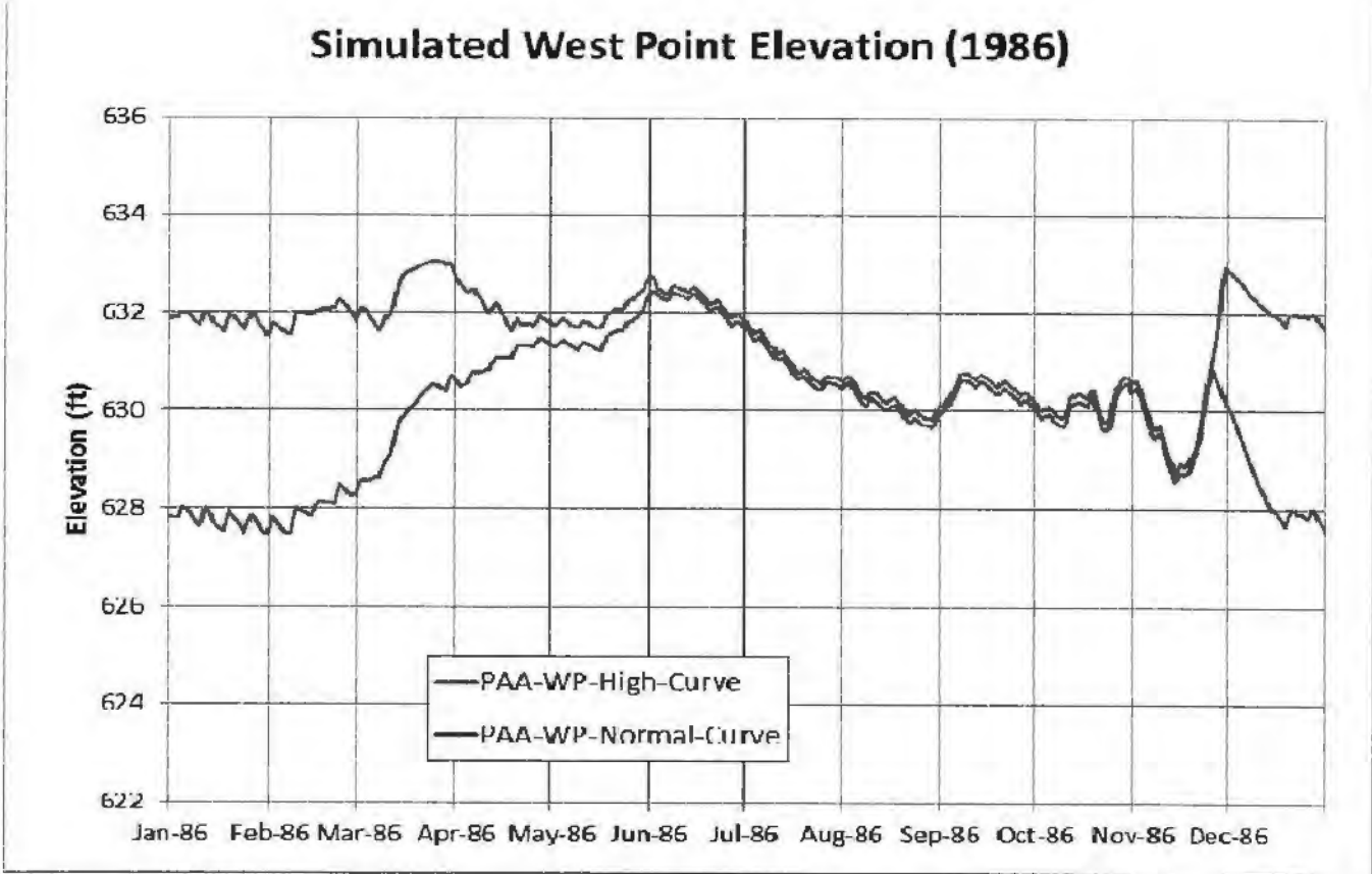
Figure 40. Simulated West Point Lake elevation in 1986.
