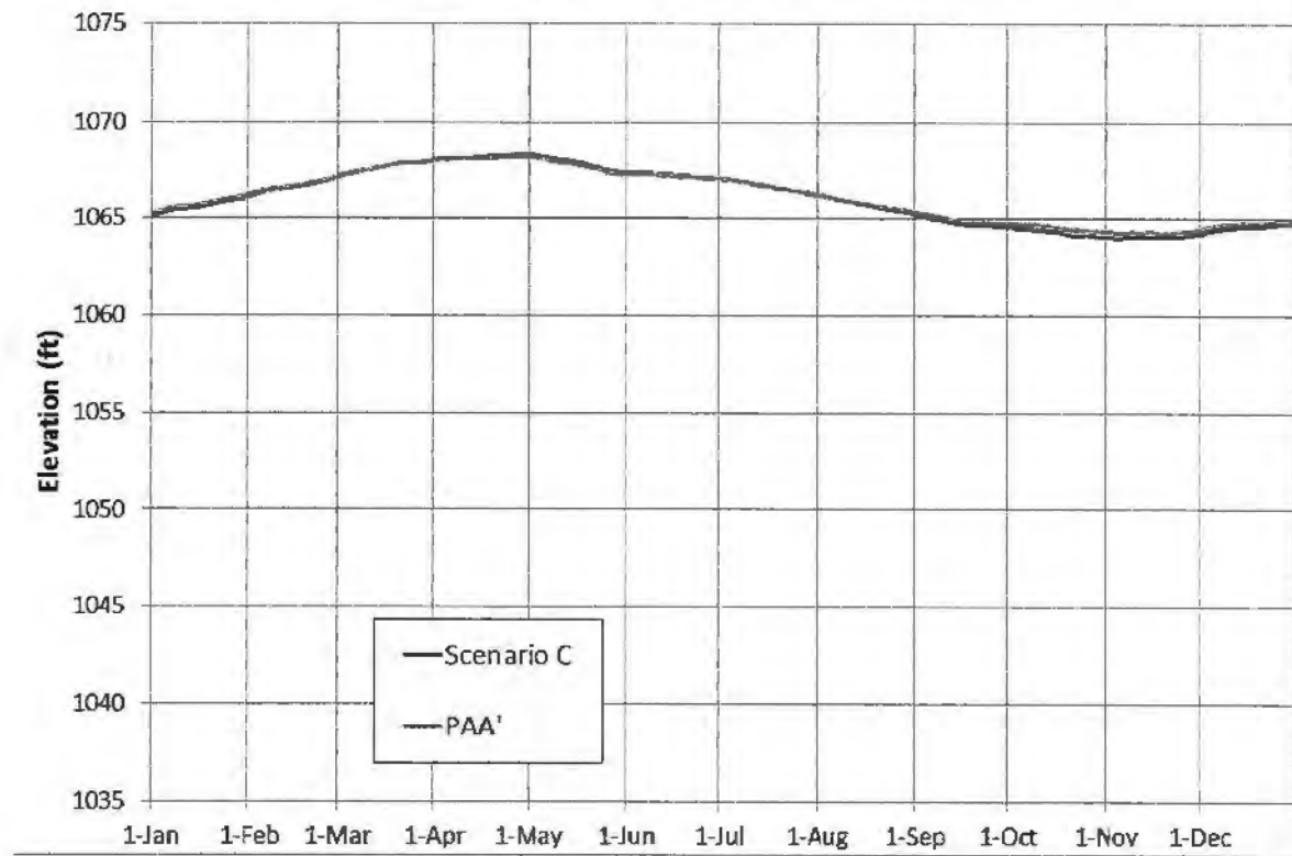
Figure 1. Simulated average daily elevation at Lake Lanier.
