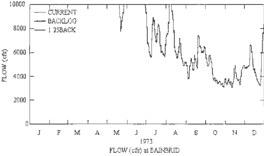
Figure I.3 - 12: Simulated streamflow of the Flint River at Bainbridge for 1973 (Wet Year)
