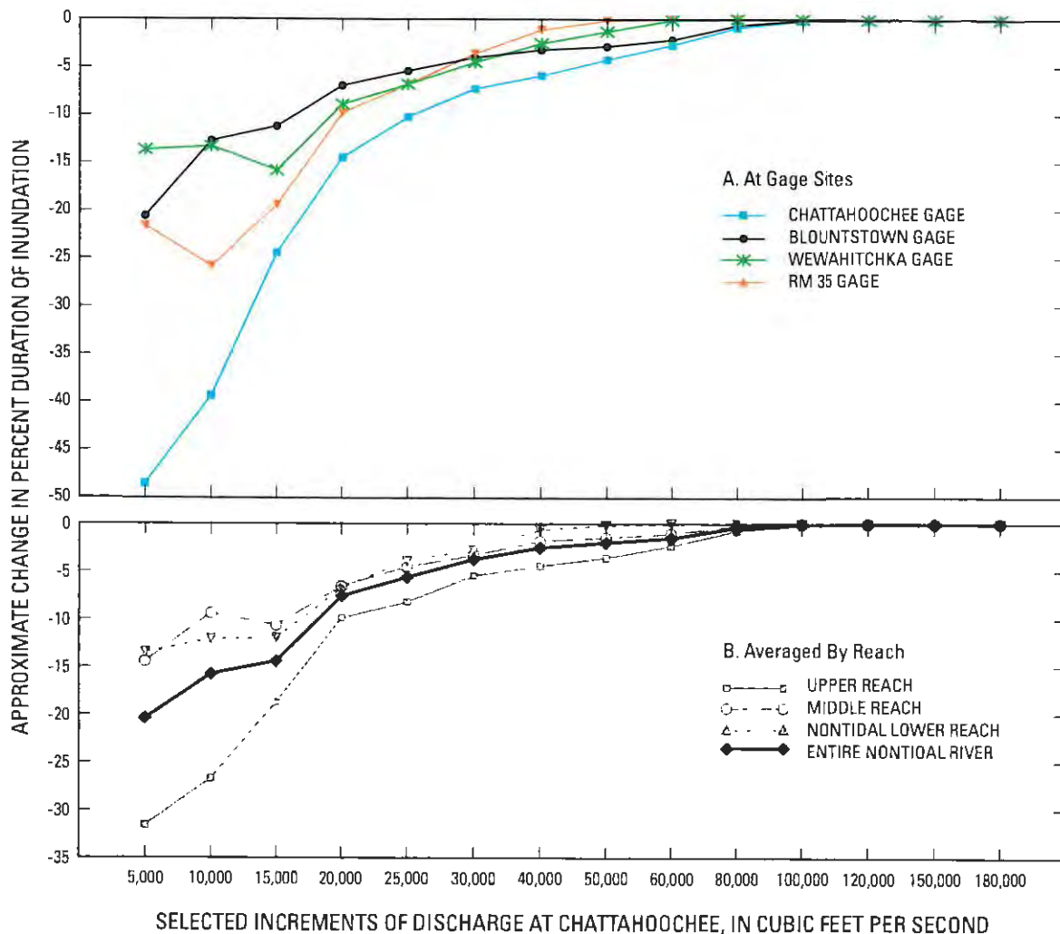
Figure 19. Approximate decreases in percent duration of inundation, at various discharges, that occurred along the nontidal Apalachicola River, Florida, as a result of long-term changes in stage-discharge relations from 1954 to 2004 (A) at streamgage sites and (B) averaged by reach. These results represent the difference between duration of inundation under actual conditions in the recent period (water years 1995–2004), reflecting the effect of water-level decline, and the duration of inundation that would have occurred in that same period if water levels had not declined. Calculations were made in a series of steps, described in the methods, starting with the pre-dam and recent stage-discharge relations. NOTE: Duration values are dependent on the time period used for calculating them (1995–2004 in this case) and would be different if a different time period were used.
