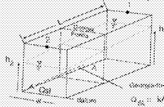
Conceptual diagram of ground-water flow across the Georgia-Florida state line
