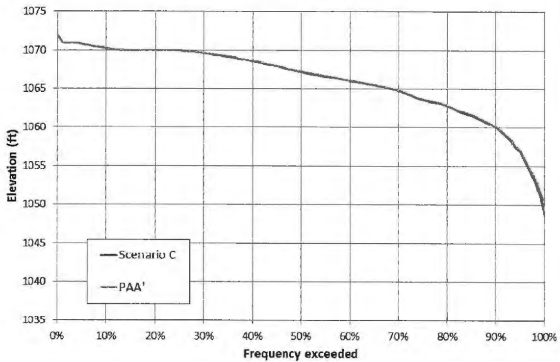
Figure 3. Duration curve of simulated Lanier elevation.
