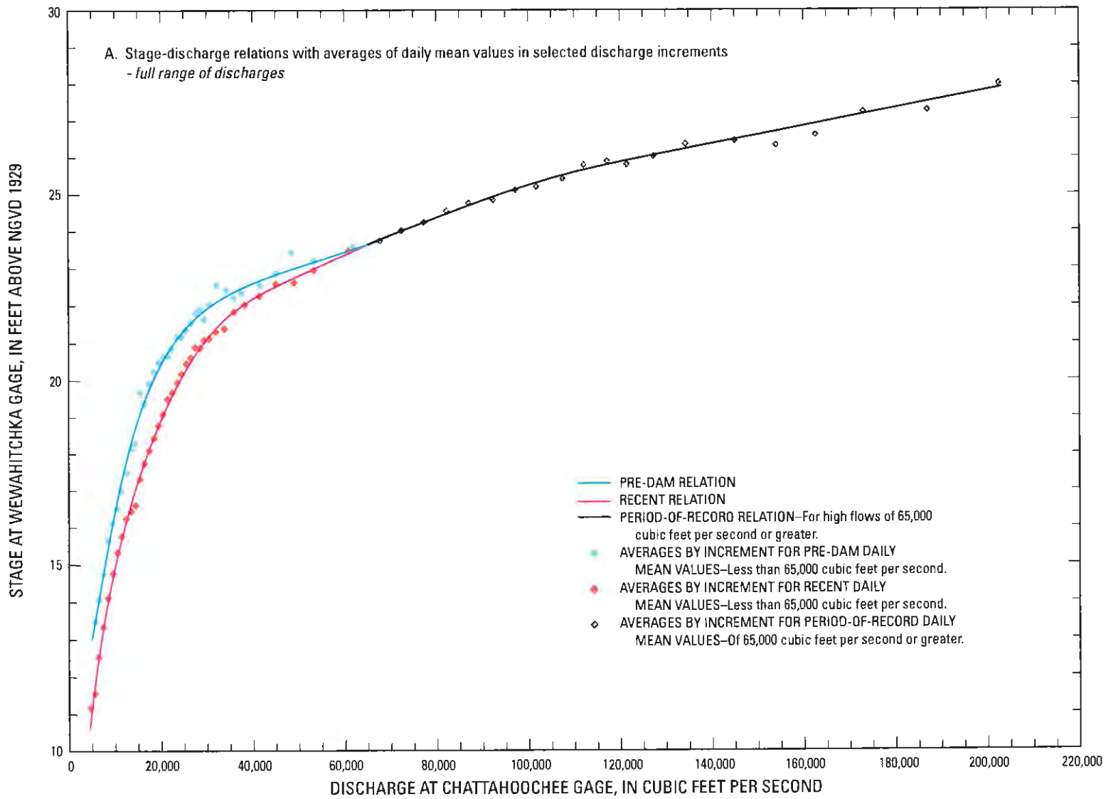
Appendix III. Stage at the Wewahitchka streamgage in relation to discharge at the Chattahoochee streamgage in the Apalachicola River, Florida. Relations were developed using a lag time of 2 days, as defined in glossary.
