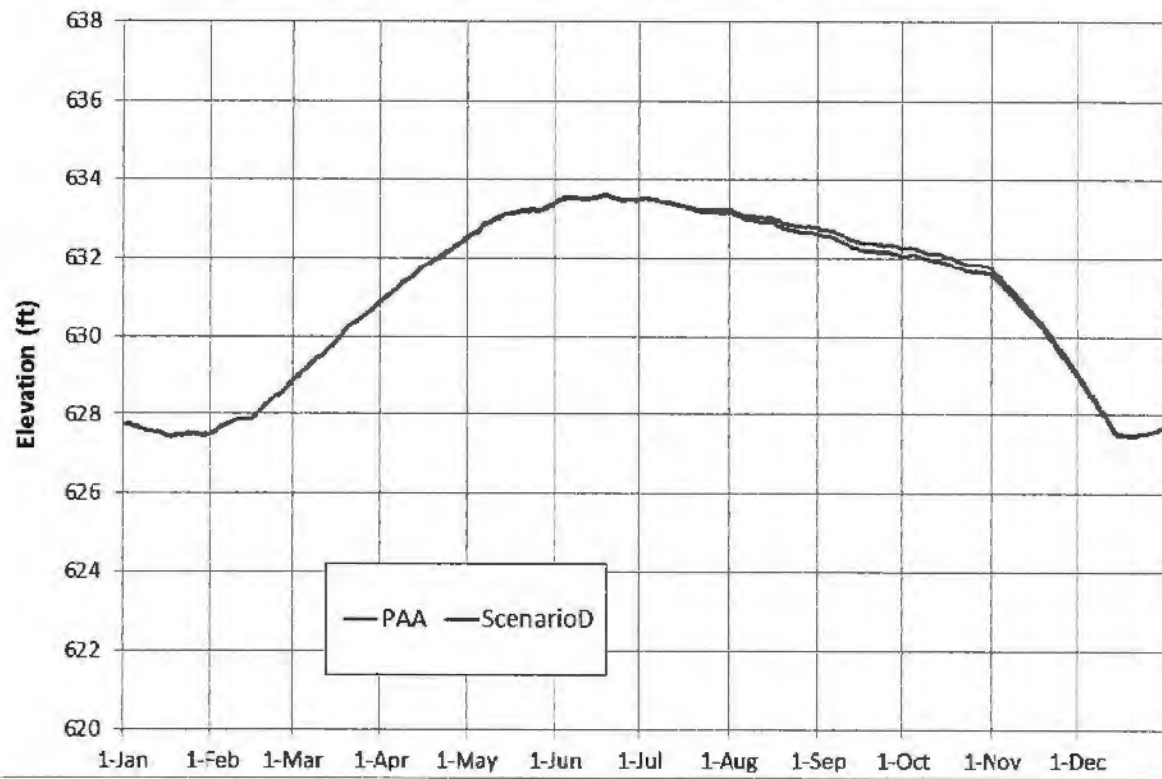
Figure 19. Simulated average daily elevation at West Point Lake
