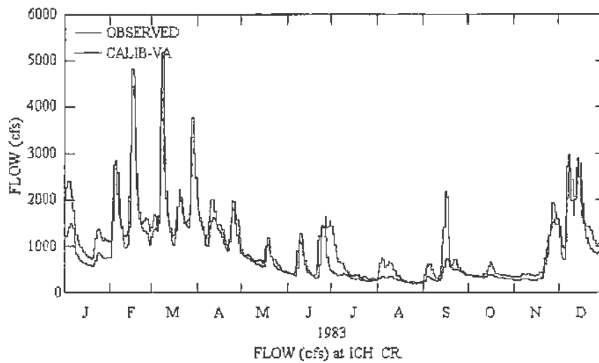
Figure 1.2 – 8: Observed vs. calibrated streamflow of Ichawaynochaway Creek near Milford for 1983 (Normal Year)
