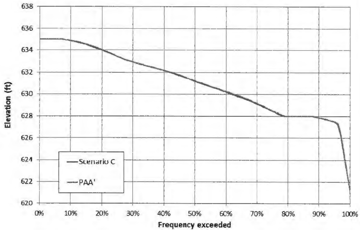
Figure 6. Duration curve of simulated West Point elevation.
