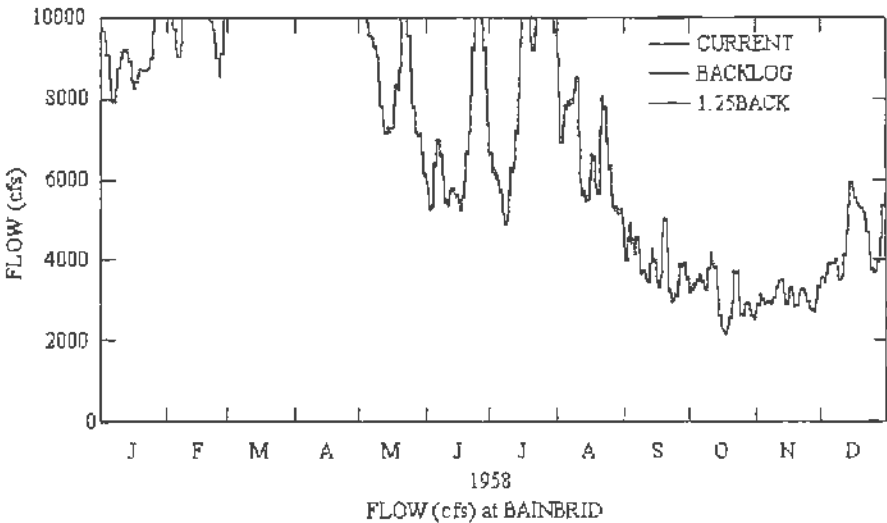
Figure I.3 - 11: Simulated streamflow of the Flint River at Bainbridge for 1958 (Normal Year)
