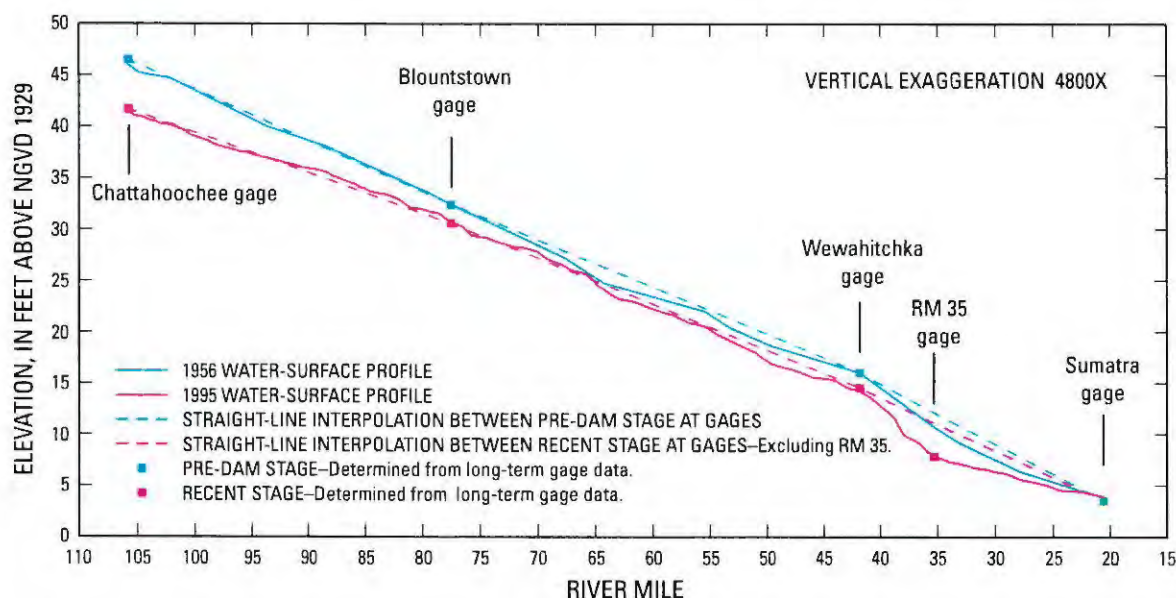
Figure 9. Comparison of water-surface profiles and stage values from long-term streamgage data for the nontidal reach of the Apalachicola River, Florida. All profile and stage data represent water levels at a Chattahoochee flow of 9,300 ft 3 /s using approximate lag times defined in glossary. Water-surface profiles were computed by U.S. Army Corps of Engineers (see fig. 4). Pre-dam and recent stages from long-term streamgage data are from stage-discharge relations developed for this report.
