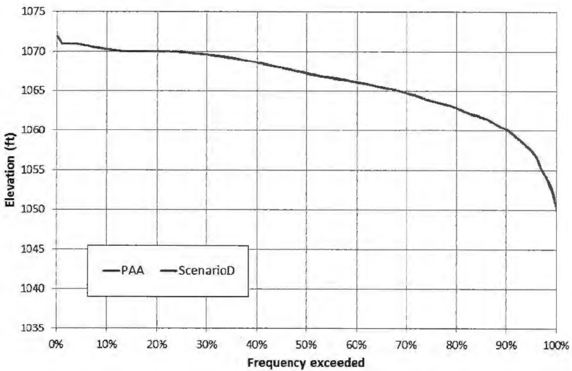
Figure 18. Duration curve of simulated Lanier elevation
