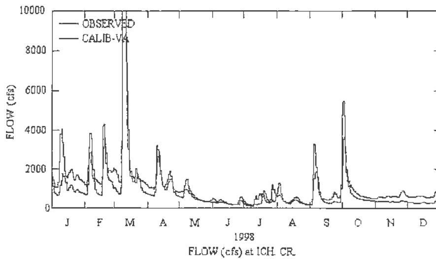
Figure 1.2 – 9: Observed vs. calibrated streamflow of Ichawaynochaway Creek near Milford for 1988 (Wet Year)
