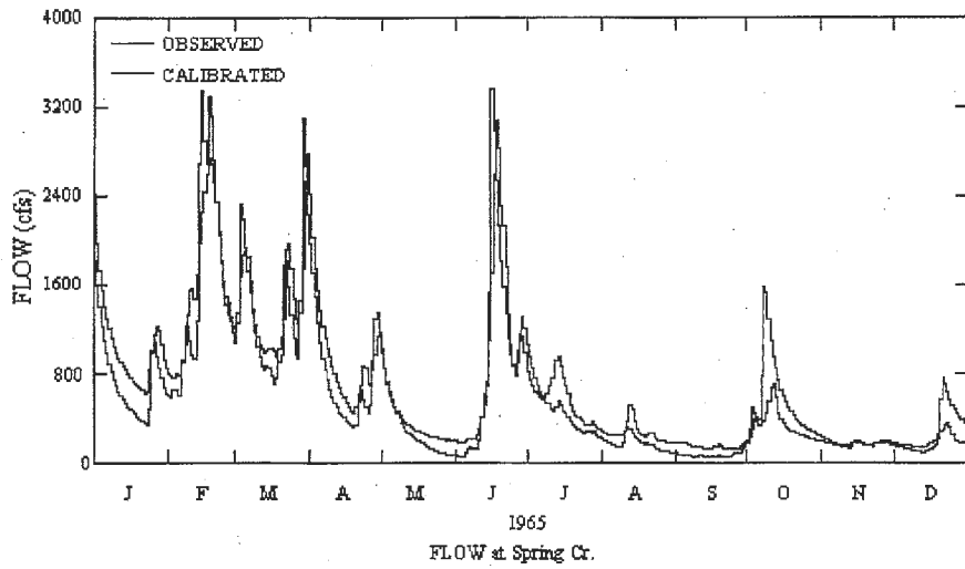
Figure I.2 – 14: Observed vs. calibrated streamflow of Spring Creek near Iron City for 1965 (Wet Year)
