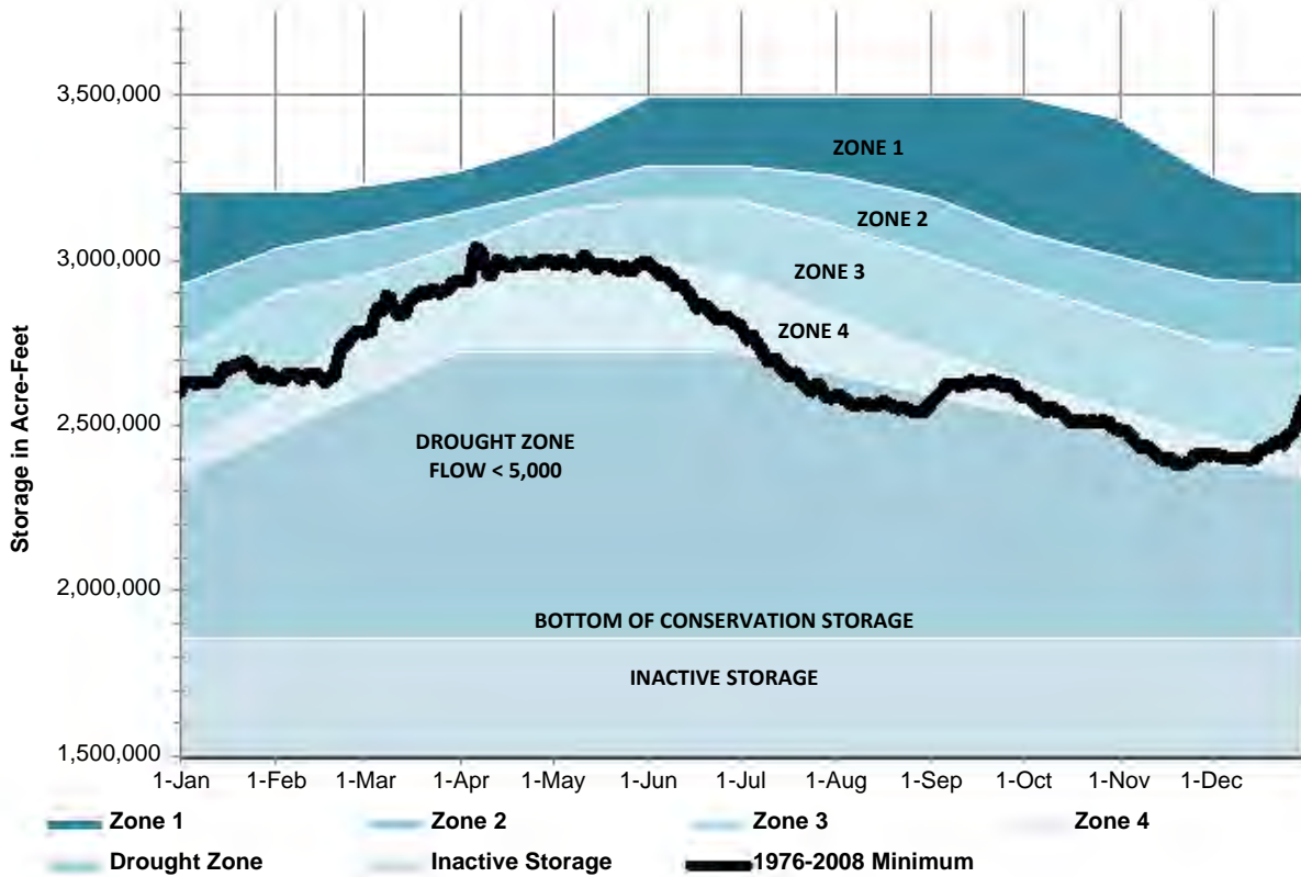
3 4 Figure 2.1-40. Basin Composite Conservation Storage and Associated Action Zones (in ac-ft)
