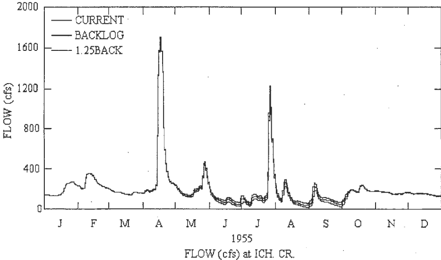
Figure I.3 – 4: Simulated streamflow of Ichawaynochaway Creek near Milford for 1955 (Dry Year)
