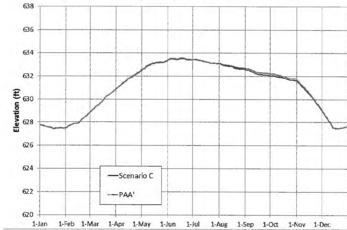
Figure 4. Simulated average daily elevation at West Point Lake.
