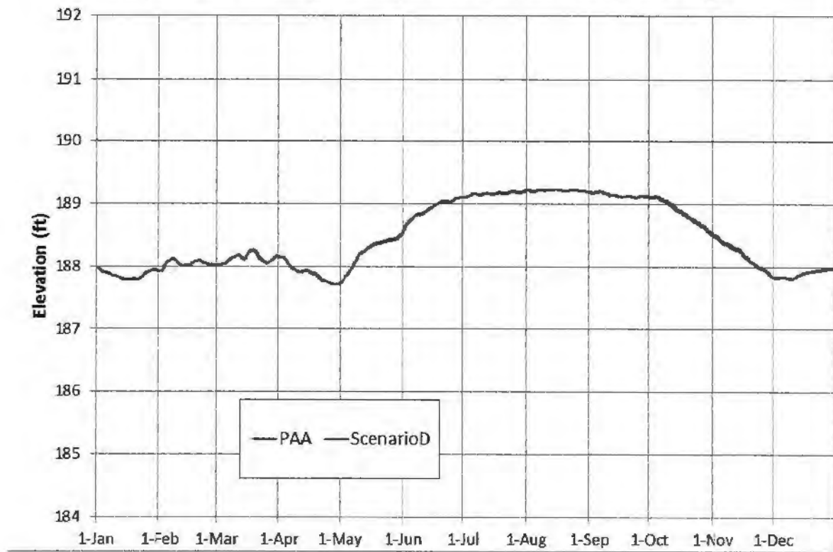
Figure 22. Simulated average daily elevation at Walter F. George Lake
