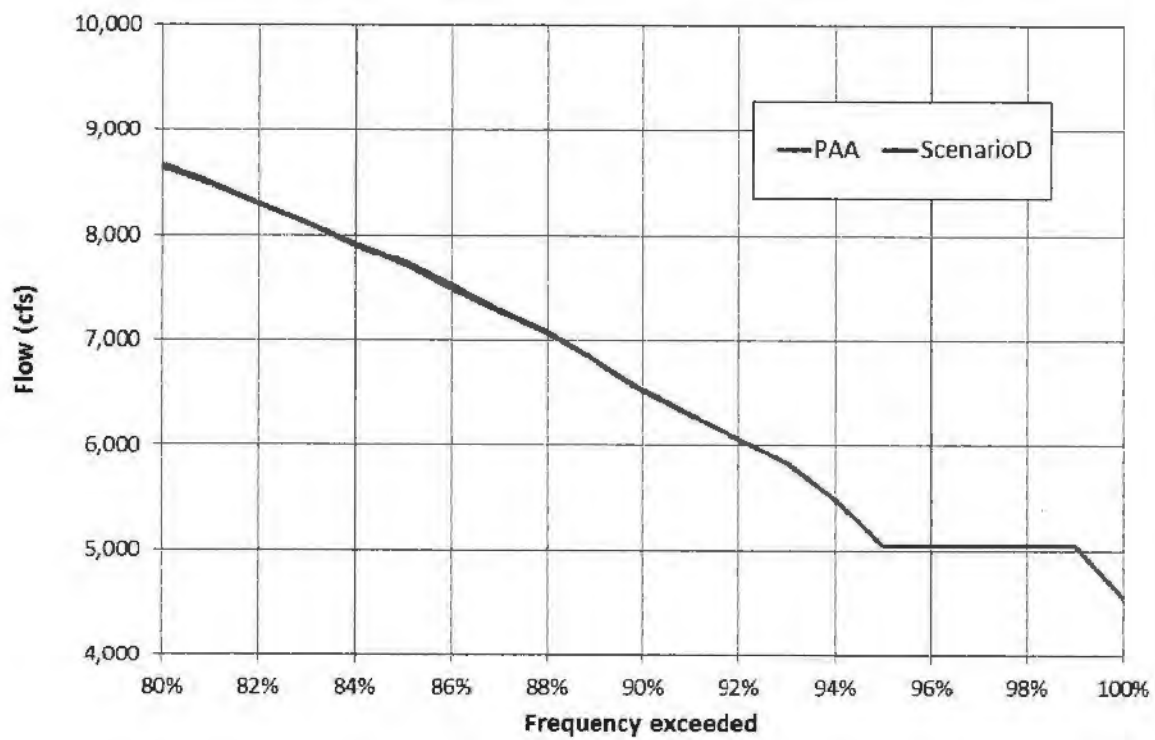
Figure 30. Duration of simulated state line flow (close-up)
